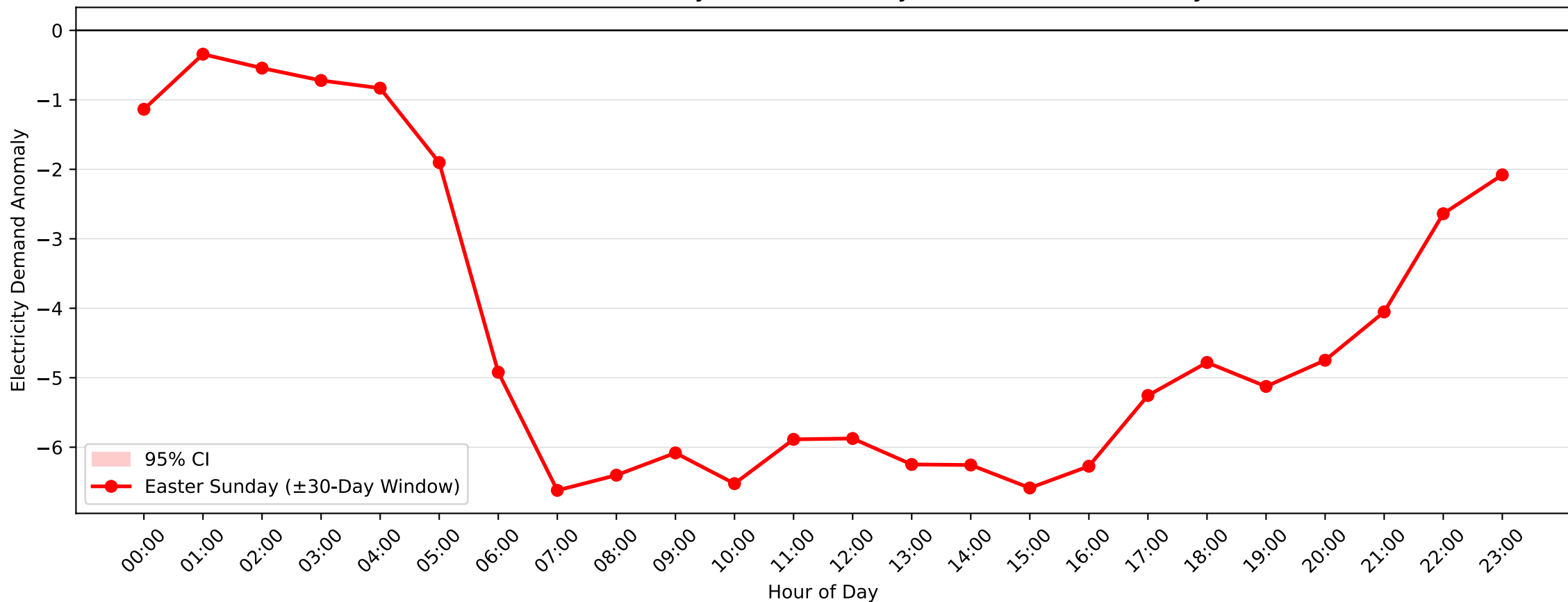
Dulwich Hill Demand Anomaly: Easter Sunday (2005–2006, \pm 30 -Day Window)
